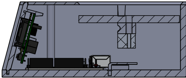
RIGHT WALL SECTION VIEW B-B
